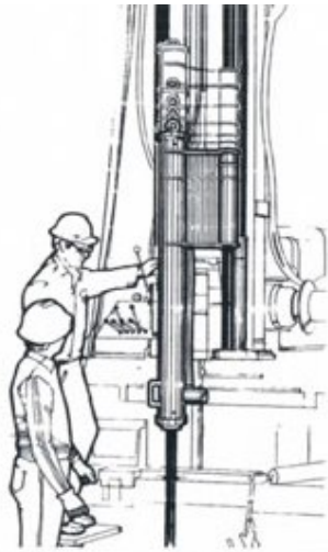
140-Pound (63.5 kg) SPT Automatic Hammer Assembly
